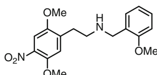
2C-N-NBOMe ( 4 ) C_{18}H_{22}N_2O_5 : 346
