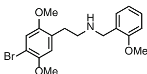
25B-NBOMe ( 3 ) C_{18}H_{22}BrNO_3 : 380
