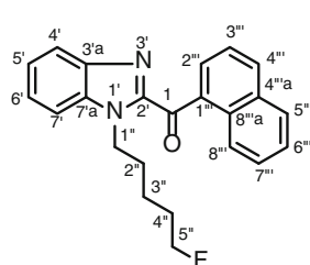
AM-2201 benzimidazole analog (1-(5-Fluoropentyl)-1 H -benzo[ d ]imidazol-2-yl)(naphthalen-1-yl)methanone (FUBIMINA, 1 ) C_{23}H_{21}FN_2O : 360
