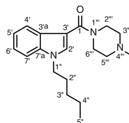
(4-Methylpiperazin-1-yl)(1-pentyl-1 H -indol-3-yl)methanone (MEPIRAPIM, 2 ) C_{19}H_{27}N_3O : 313
