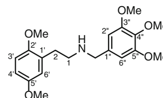
25H-NBOMe 3,4,5-trimethoxybenzyl analog ( 5 ) 2-(2,5-Dimethoxyphenyl)- N -(3,4,5-trimethoxybenzyl)ethanamine C_{20}H_{27}NO_5 : 361
