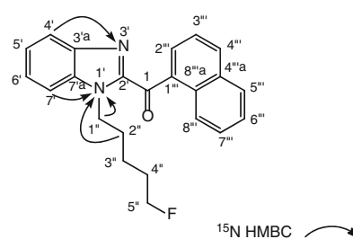
(b) Compound (1)
