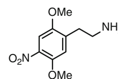
25H-NBOMe 3,4,5-trimethoxybenzyl analog ( 5 ) 2-(2,5-Dimethoxyphenyl)- N -(3,4,5-trimethoxybenzyl)ethanamine C_{20}H_{27}NO_5 : 361
